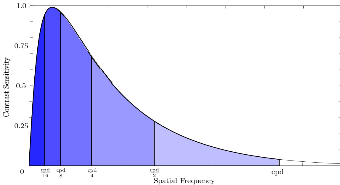
Figure 1: Device and viewing condition-dependent parameters based multi-scale weights calculation scheme
