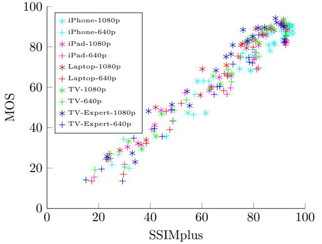
Figure 7: MOS versus SSIMplus scatter plot
