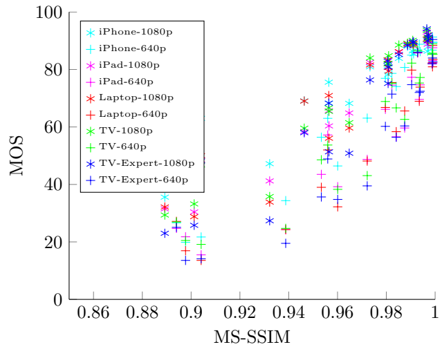
Figure 4: MOS versus MS-SSIM scatter plot
