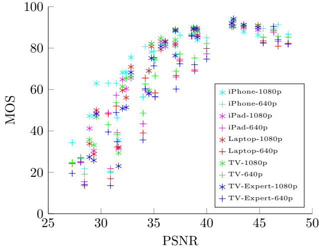
Figure 2: MOS versus PSNR scatter plot
