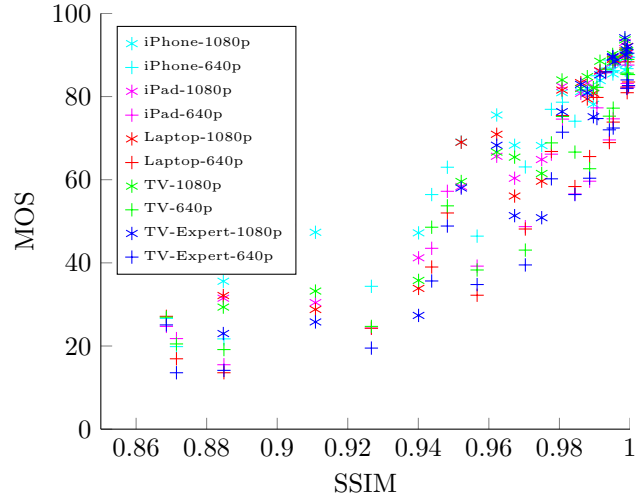
Figure 3: MOS versus SSIM scatter plot
