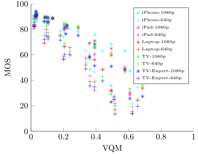
Figure 5: MOS versus VQM scatter plot
