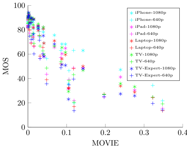
Figure 6: MOS versus MOVIE scatter plot
