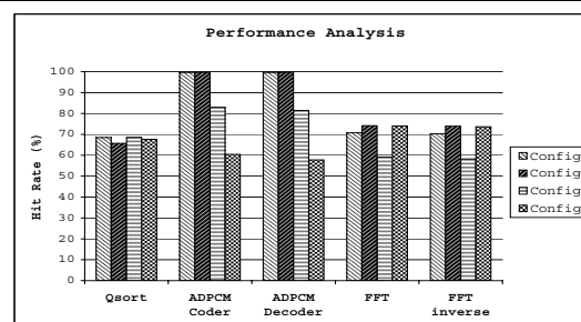
Figure 3. Performance of media benchmarks.
