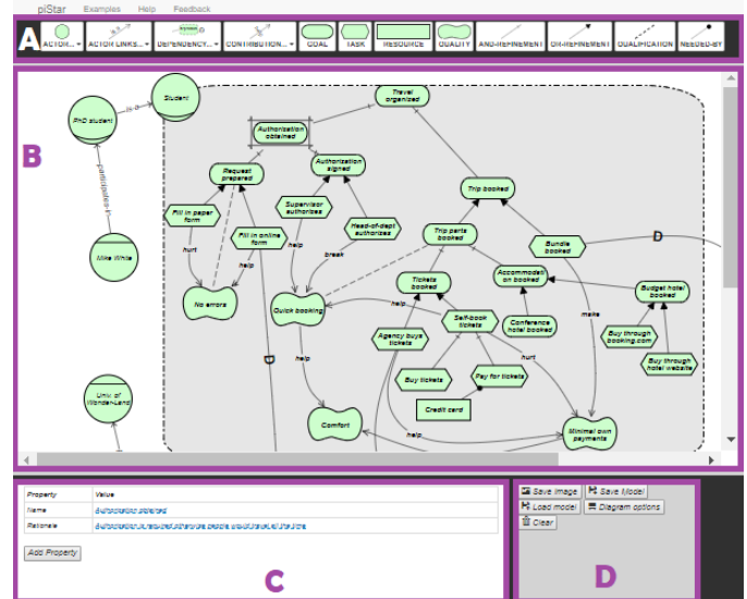
Fig. 1. A screenshot of the piStar tool
