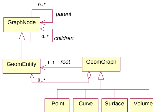
Figure 5-5 Geometry Participants (Brep graph)
