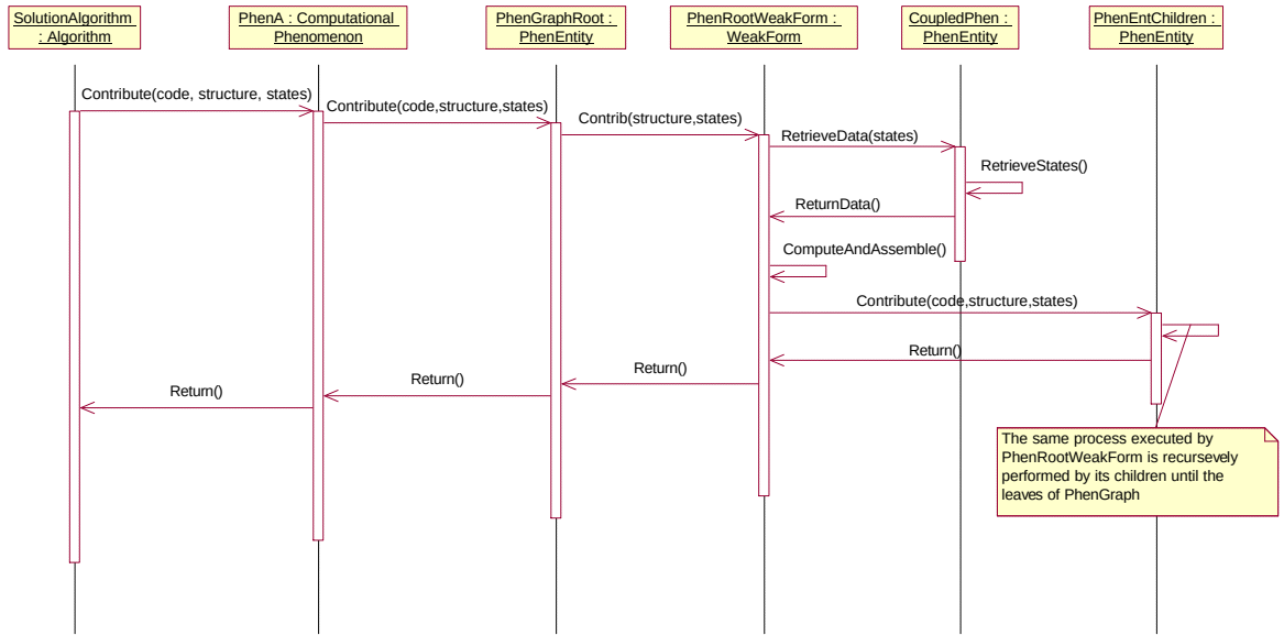
Figure 5-8 Sequence diagram for Computational Phenomenon
