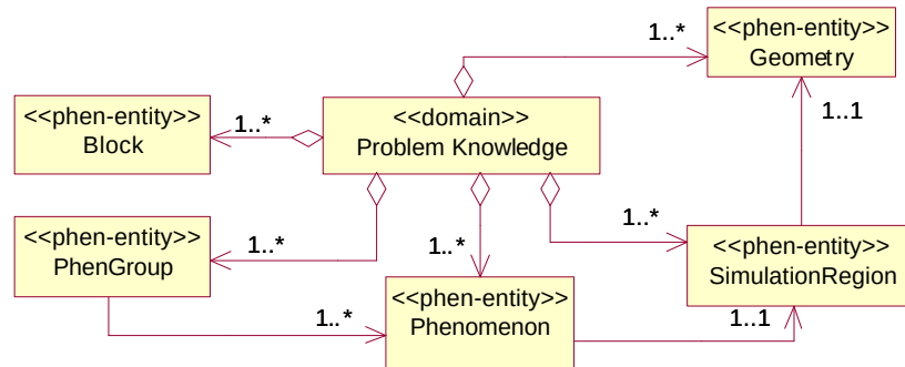
Figure 3-18 Problem Knowledge Domain
