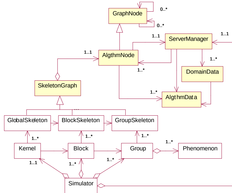
Figure 4-8 Simulator Component
