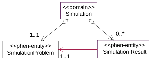
Figure 3-22 Simulation Domain
