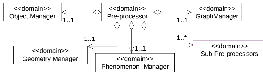
Figure 3-21 Pre-processor Domain
