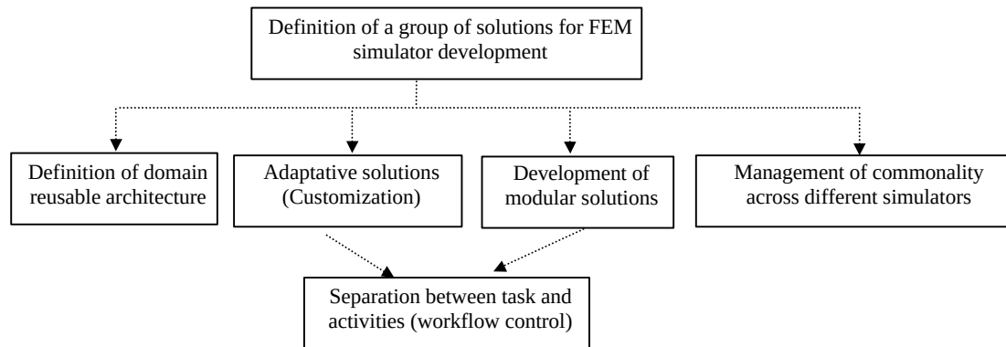
Figure 3-8 Solutions Decomposition
