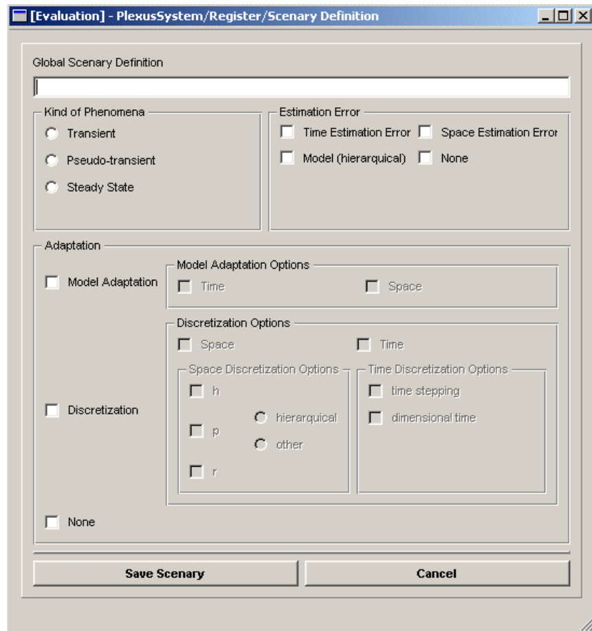
Figure C-12 Global Scenario
