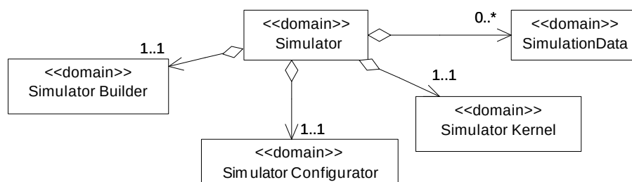
Figure 3-19 Simulator Domain
