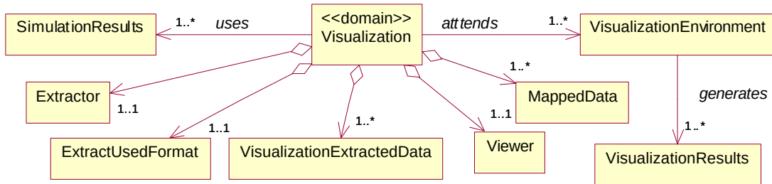
Figure 3-23 Visualization Domain
