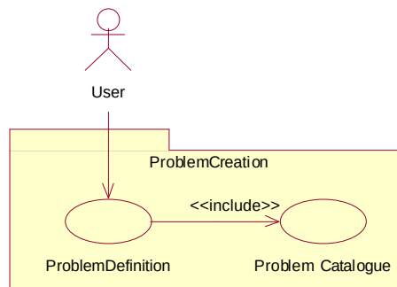
Figure C-7 Problem Creation
