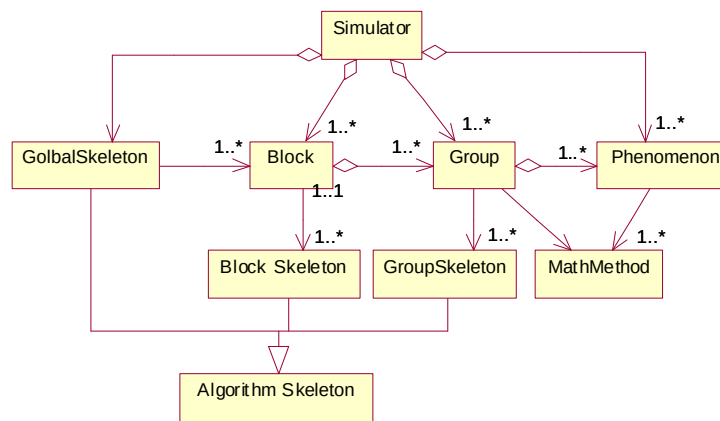
Figure 5-13 Participants of the Simulator Pattern
