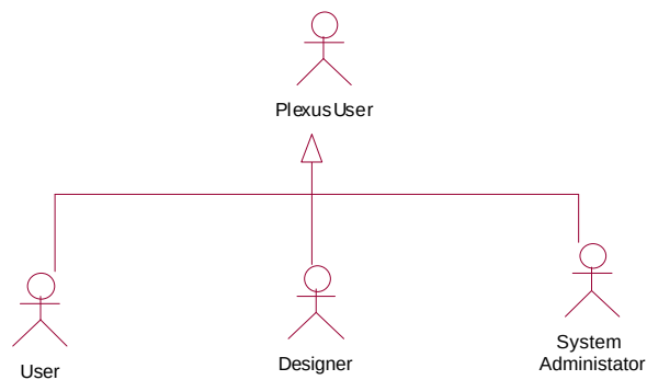
Figure C-4 Existing actors
