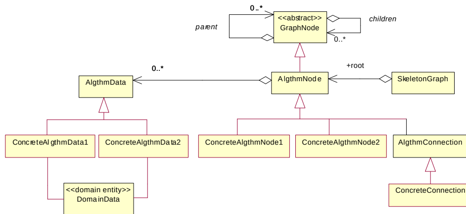
Figure 5-19 Participants of the GIG-pattern
