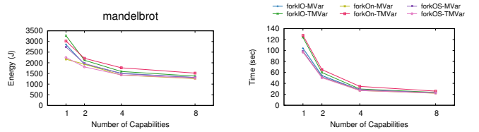
Fig. 6. Energy/Time on Alternative Platform
