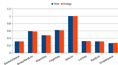
Fig. 4. Results of remove operation for Sequences
