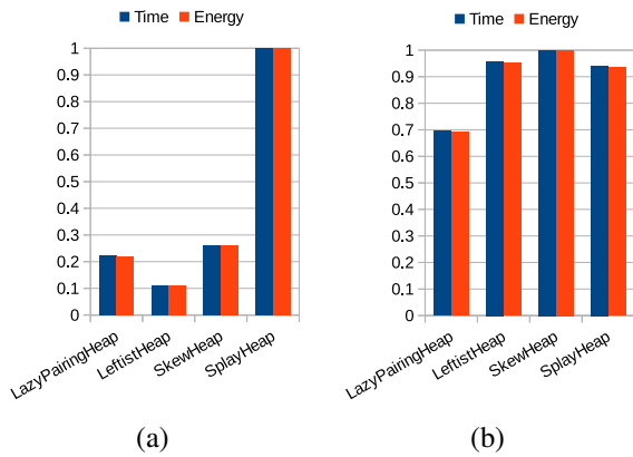
Fig. 2. Results of add and toList operations for Heaps
